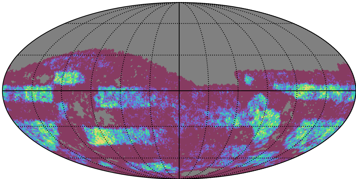
no_magell_roll_v3.4_10yrs Yr 3-4 g band: NVisits
