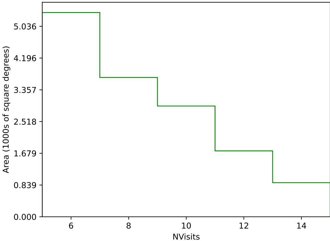
no_magell_roll_v3.4_10yrs Yr 3-4 g band: NVisits
