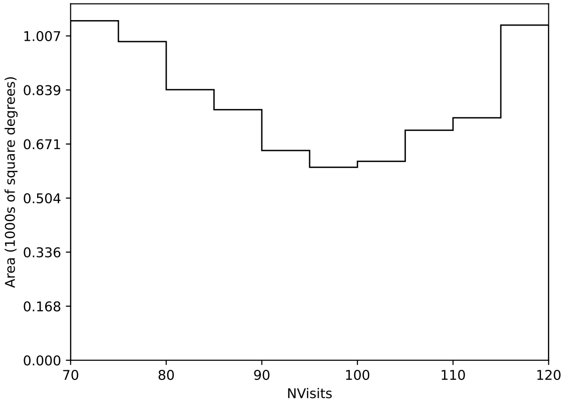
no_magell_roll_v3.4_10yrs Yr 3-4 all bands: NVisits
