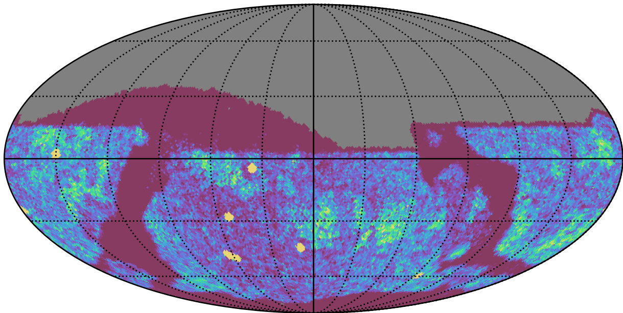
no_magell_roll_v3.4_10yrs Yr 1 z band: NVisits
