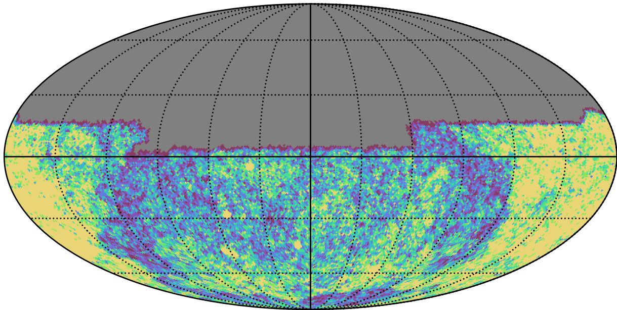
no_magell_roll_v3.4_10yrs Yr 1 u band: NVisits
