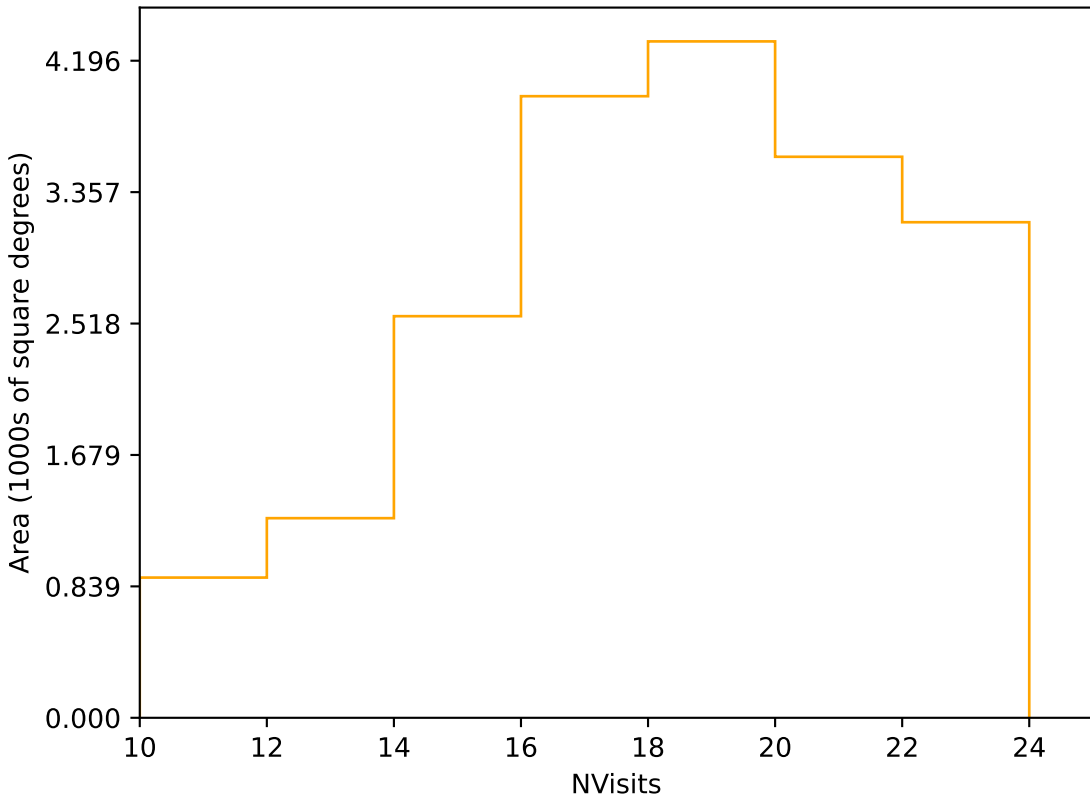
no_magell_roll_v3.4_10yrs Yr 1 r band: NVisits
