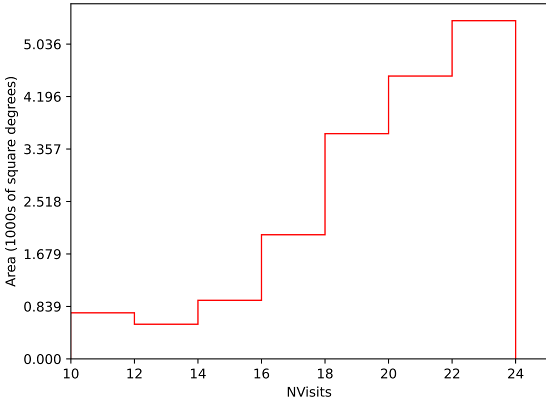
no_magell_roll_v3.4_10yrs Yr 1 i band: NVisits
