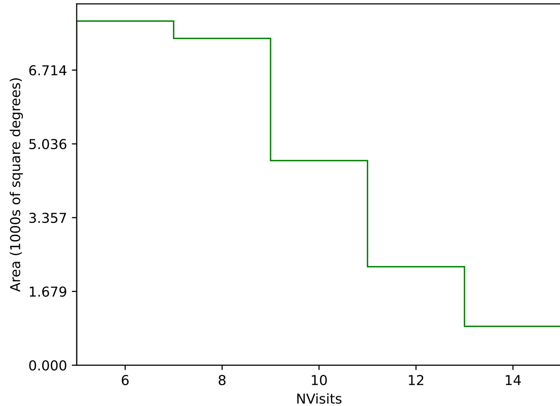
no_magell_roll_v3.4_10yrs Yr 1 g band: NVisits
