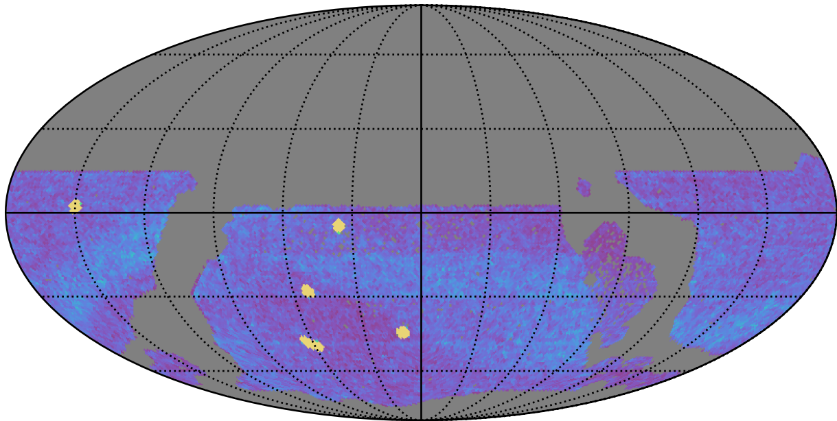
no_magell_roll_v3.4_10yrs WFD all bands: NVisits
