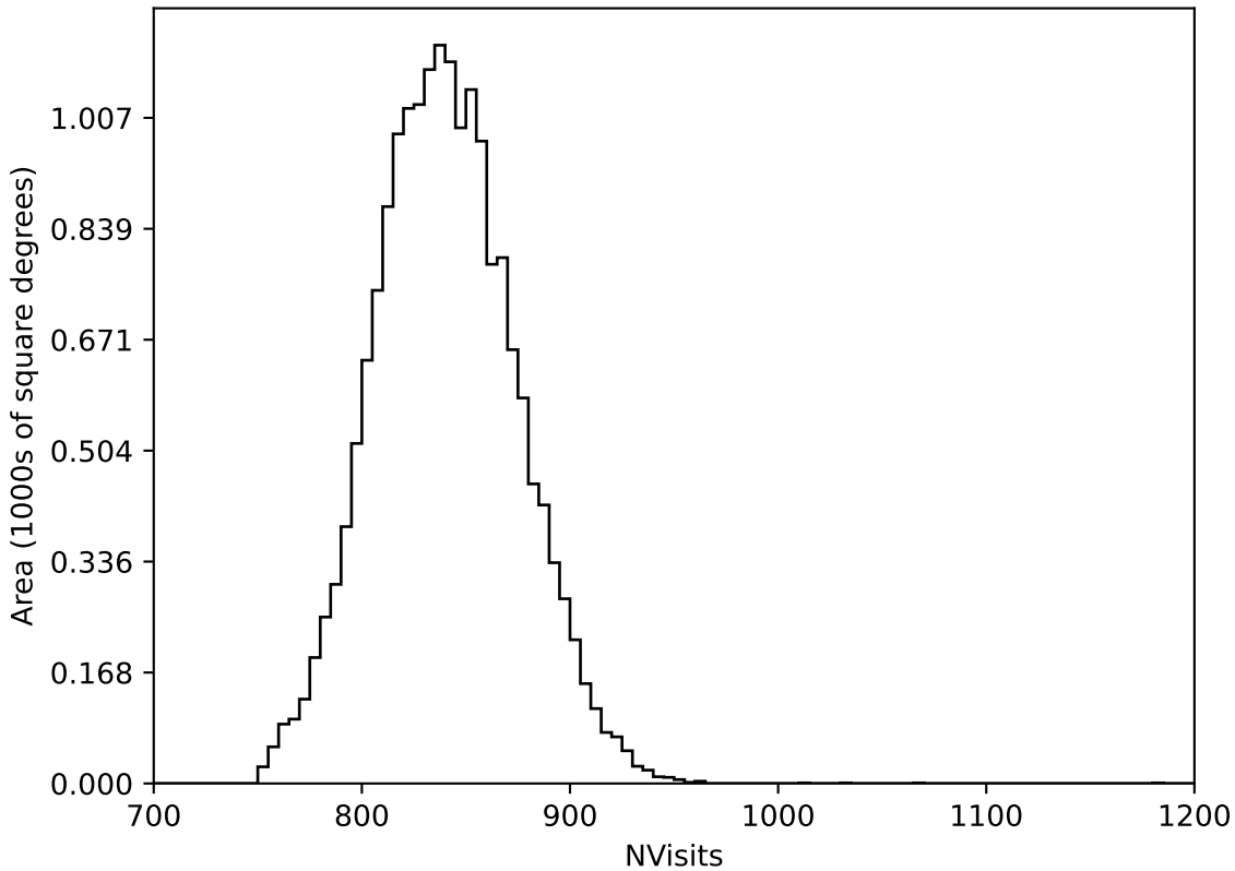
no_magell_roll_v3.4_10yrs WFD all bands: NVisits
