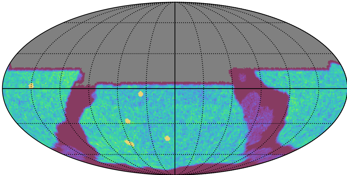
no_magell_roll_v3.4_10yrs All sky u band: NVisits
