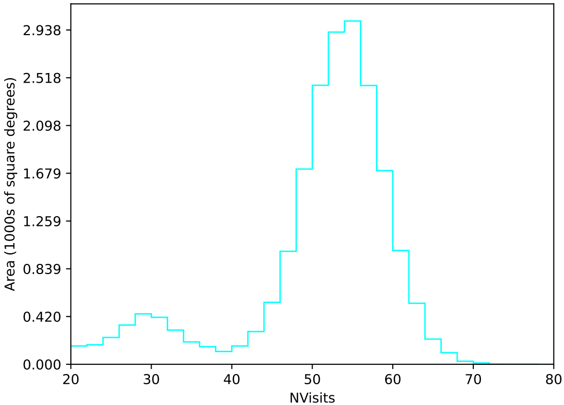
no_magell_roll_v3.4_10yrs All sky u band: NVisits
