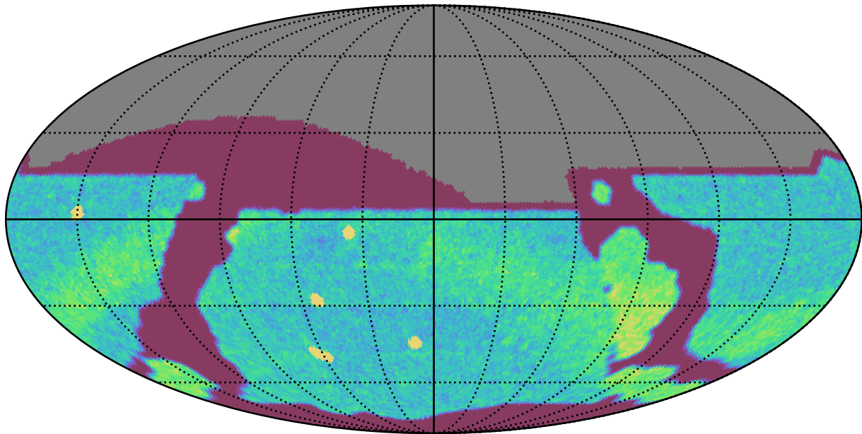
no_magell_roll_v3.4_10yrs All sky r band: NVisits
