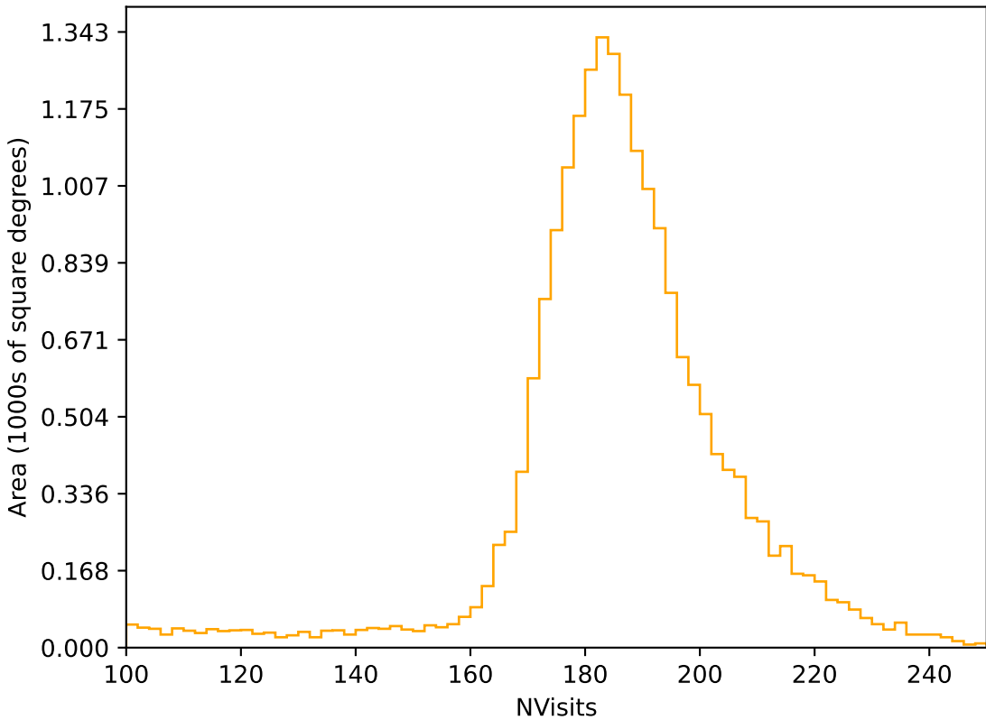
no_magell_roll_v3.4_10yrs All sky r band: NVisits
