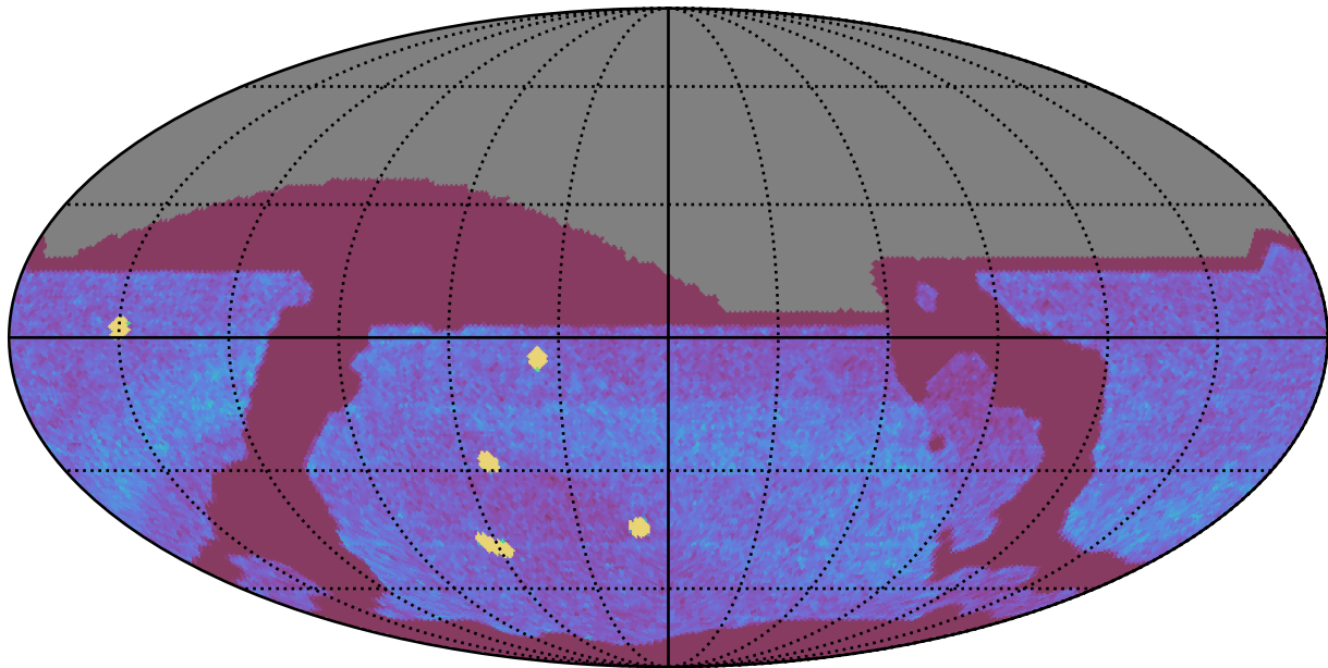
no_magell_roll_v3.4_10yrs All sky all bands: NVisits
