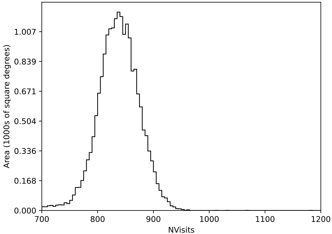
no_magell_roll_v3.4_10yrs All sky all bands: NVisits
