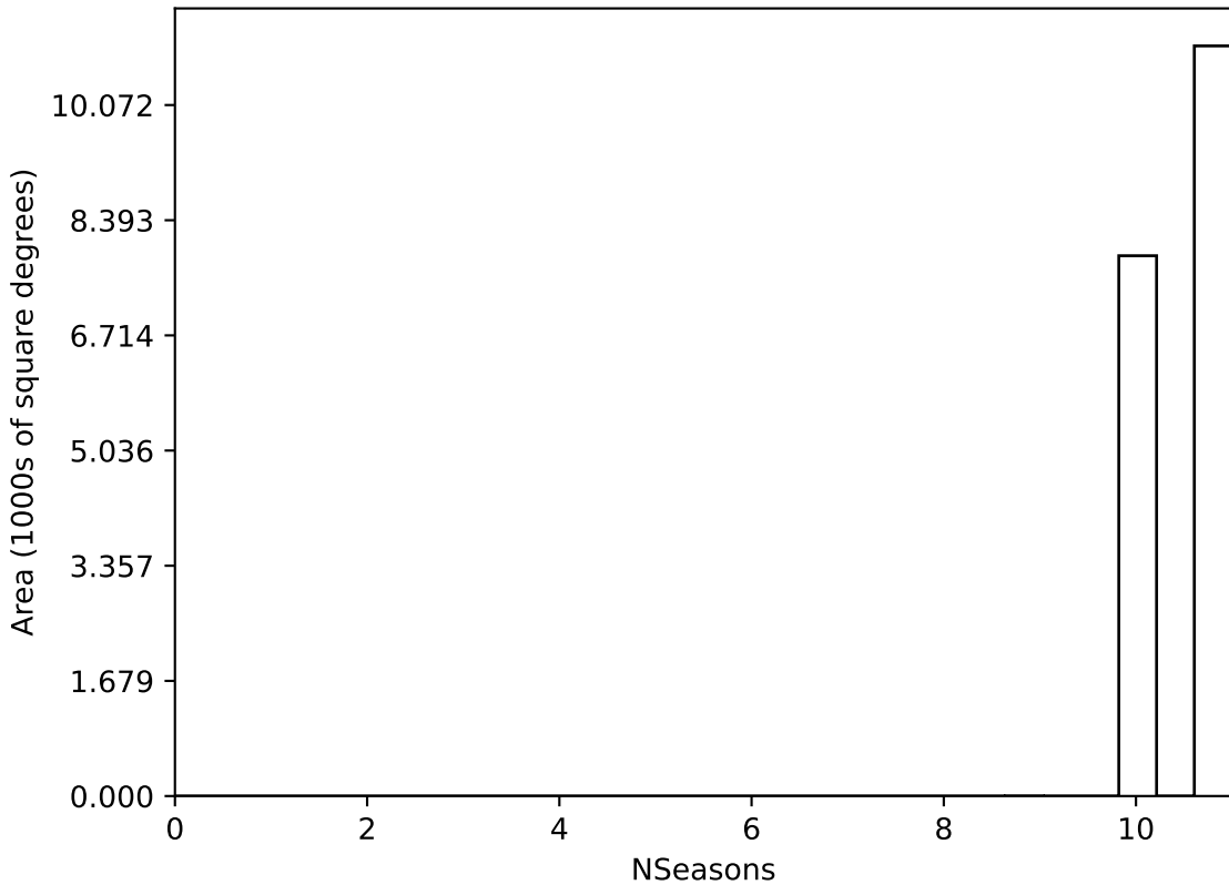
no_magell_roll_v3.4_10yrs WFD all bands: NSeasons
