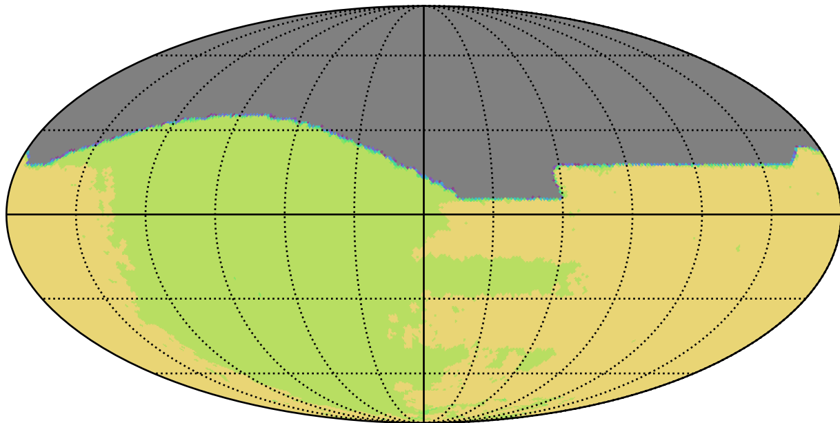
no_magell_roll_v3.4_10yrs All sky all bands: NSeasons
