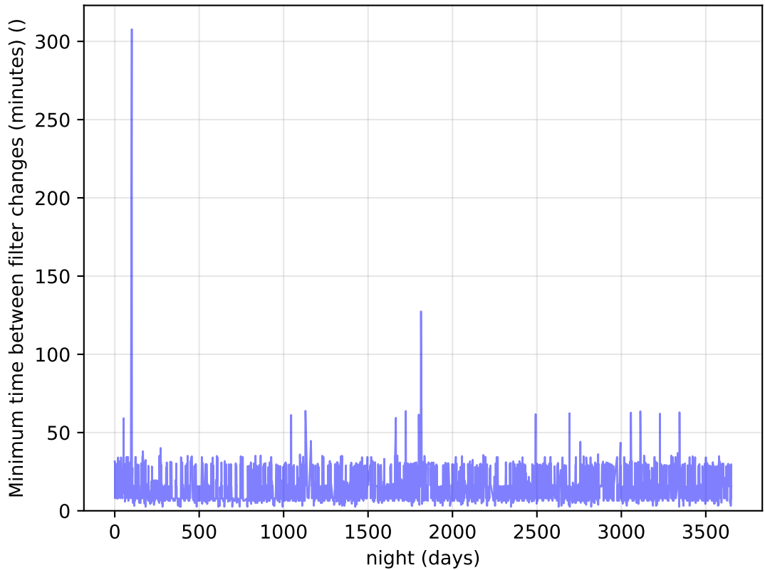
no_magell_roll_v3.4_10yrs Per Night: Minimum time between filter changes (minutes)
