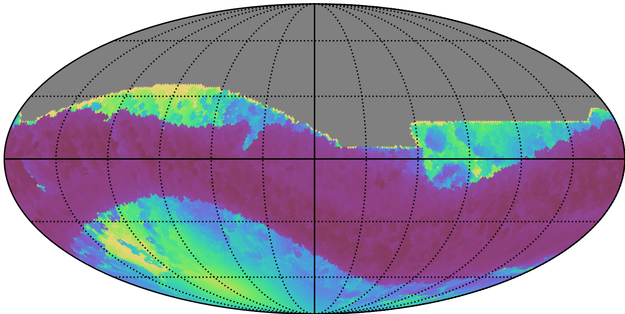
no_magell_roll_v3.4_10yrs All sky all bands: Min solarElong
