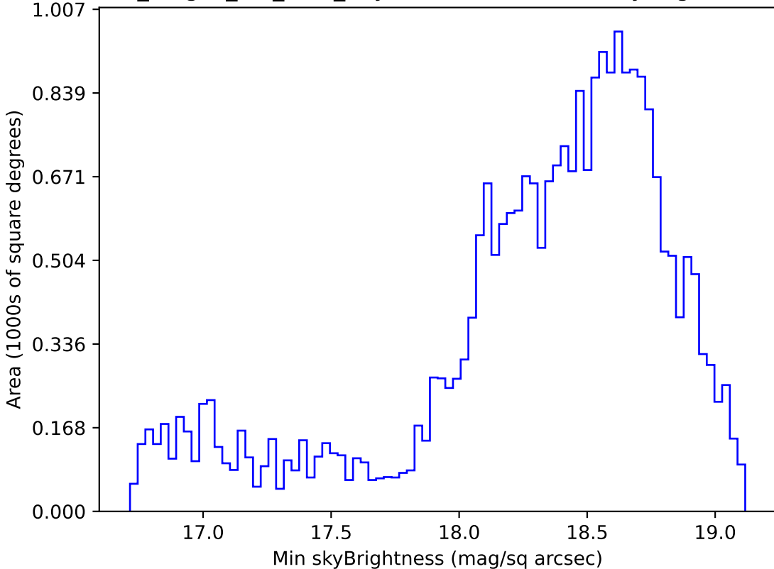
no_magell_roll_v3.4_10yrs Yr 1 z band: Min skyBrightness
