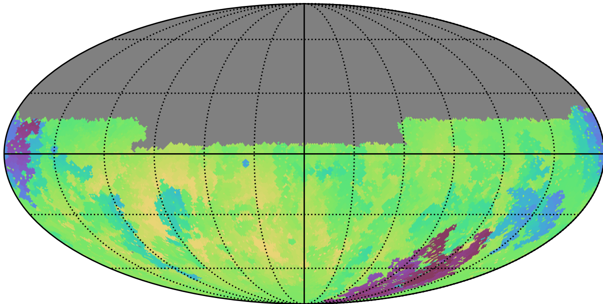
no_magell_roll_v3.4_10yrs Yr1 u band: Min skyBrightness
