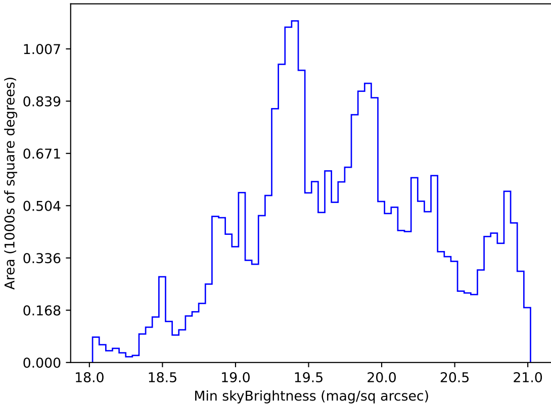
no_magell_roll_v3.4_10yrs Yr 1 r band: Min skyBrightness
