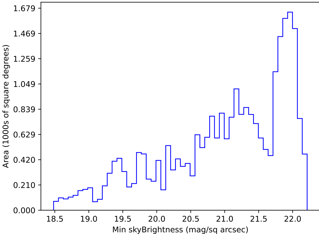
no_magell_roll_v3.4_10yrs Yr 1 g band: Min skyBrightness
