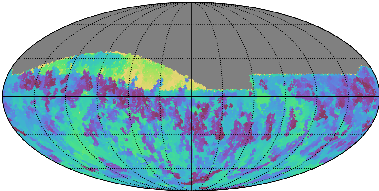
no_magell_roll_v3.4_10yrs Yr 1 all bands: Min skyBrightness
