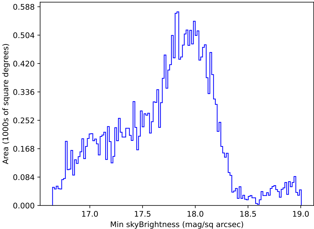
no_magell_roll_v3.4_10yrs Yr 1 all bands: Min skyBrightness
