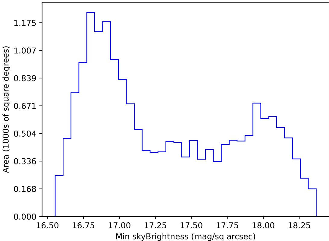
no_magell_roll_v3.4_10yrs WFD z band: Min skyBrightness
