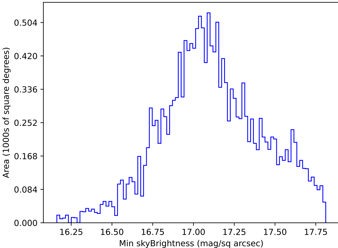
no_magell_roll_v3.4_10yrs WFD y band: Min skyBrightness
