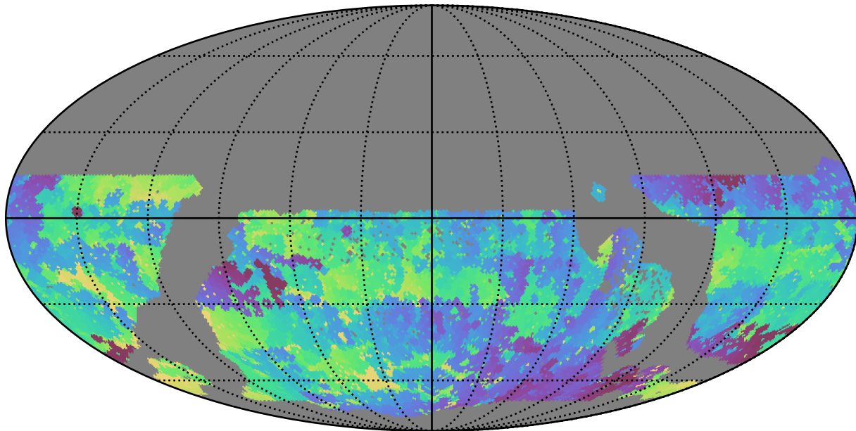
no_magell_roll_v3.4_10yrs WFD u band: Min skyBrightness
