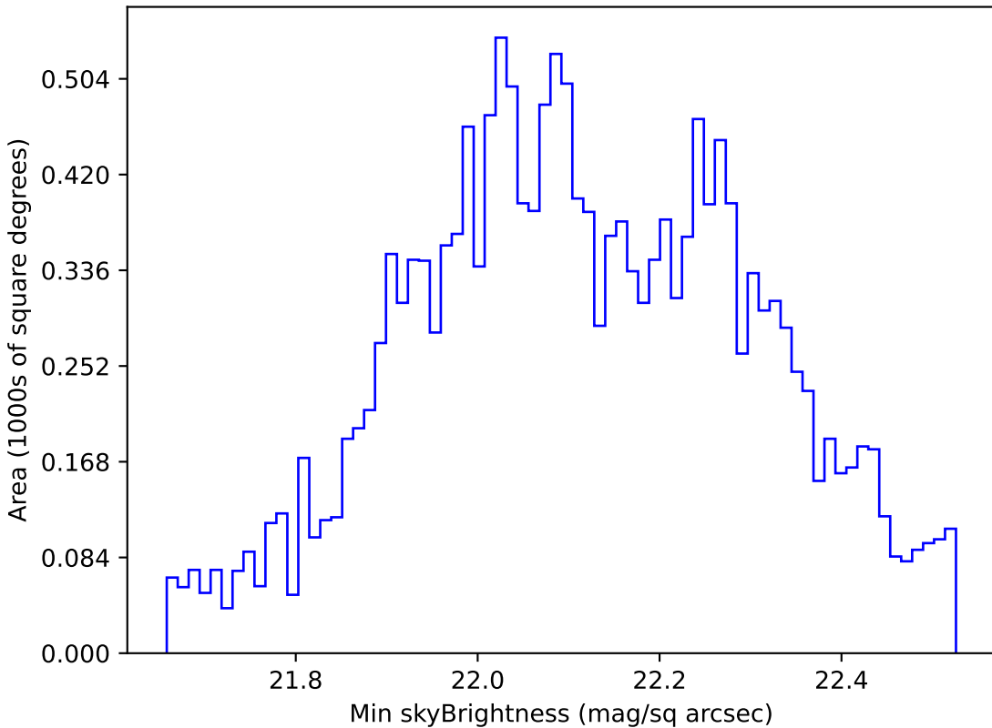
no_magell_roll_v3.4_10yrs WFD u band: Min skyBrightness
