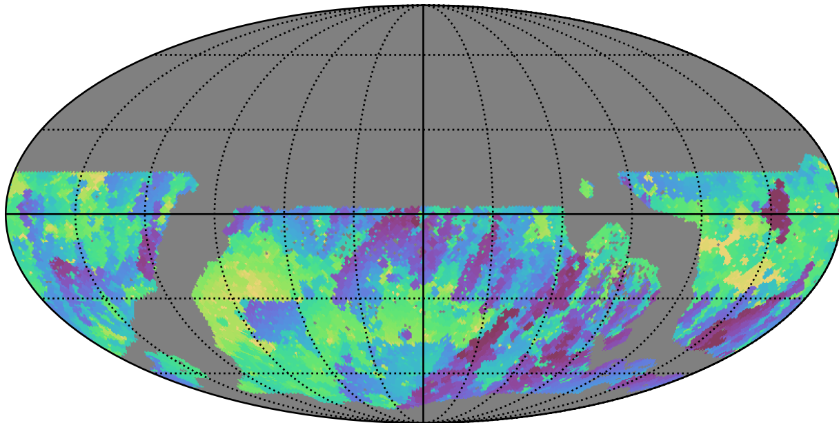
no_magell_roll_v3.4_10yrs WFD r band: Min skyBrightness
