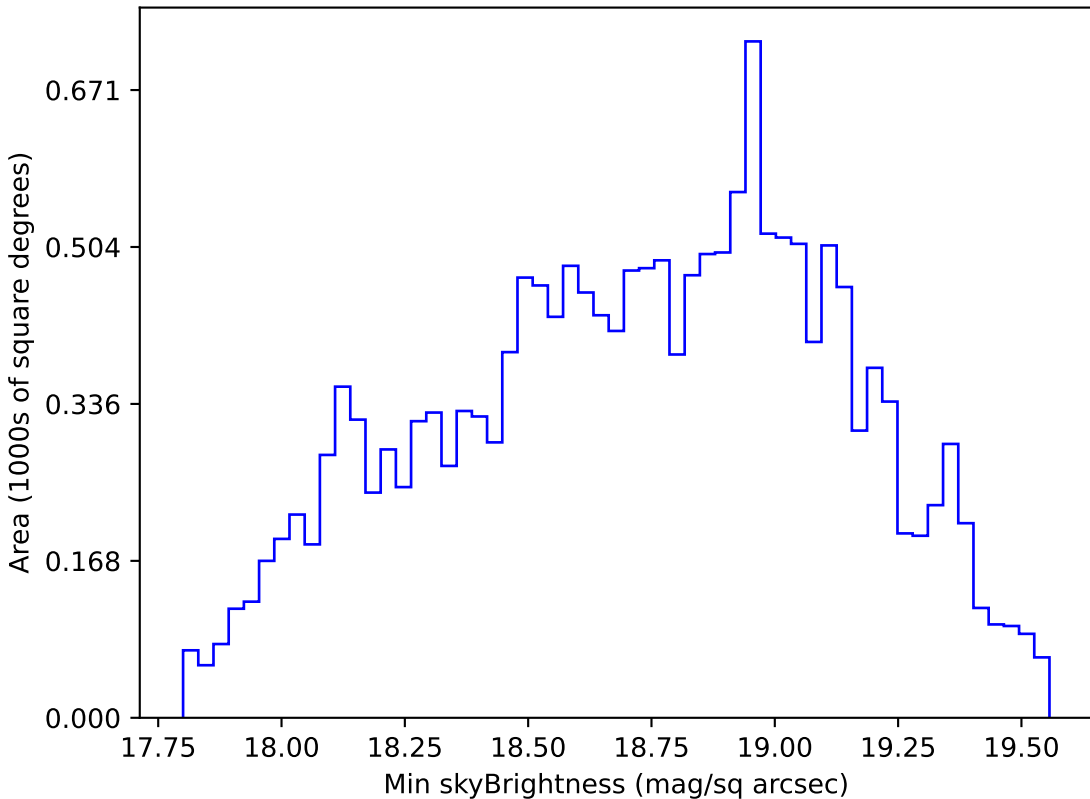
no_magell_roll_v3.4_10yrs WFD r band: Min skyBrightness
