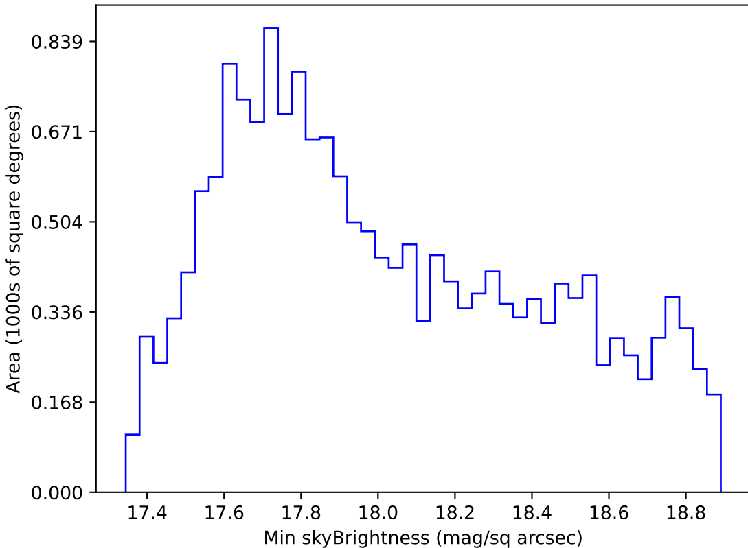
no_magell_roll_v3.4_10yrs WFD i band: Min skyBrightness
