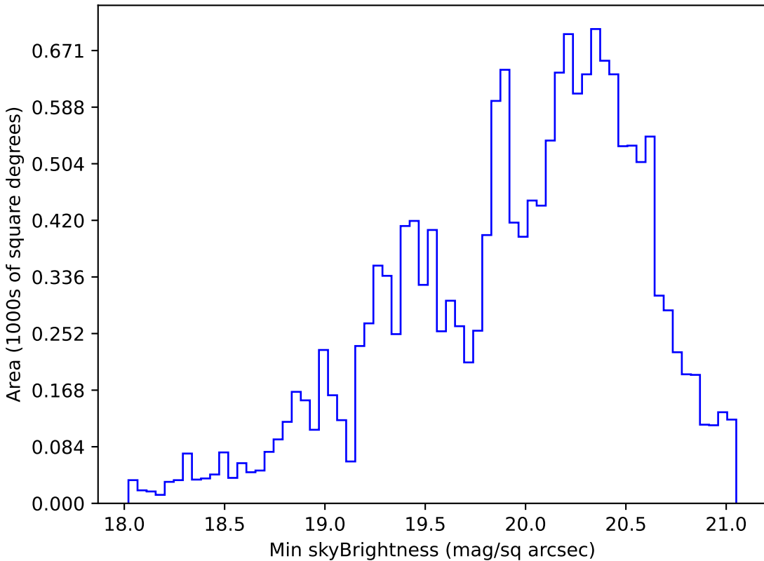
no_magell_roll_v3.4_10yrs WFD g band: Min skyBrightness
