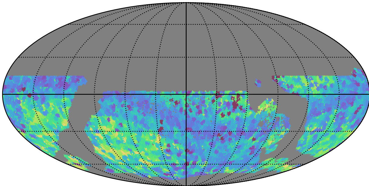
no_magell_roll_v3.4_10yrs WFD all bands: Min skyBrightness
