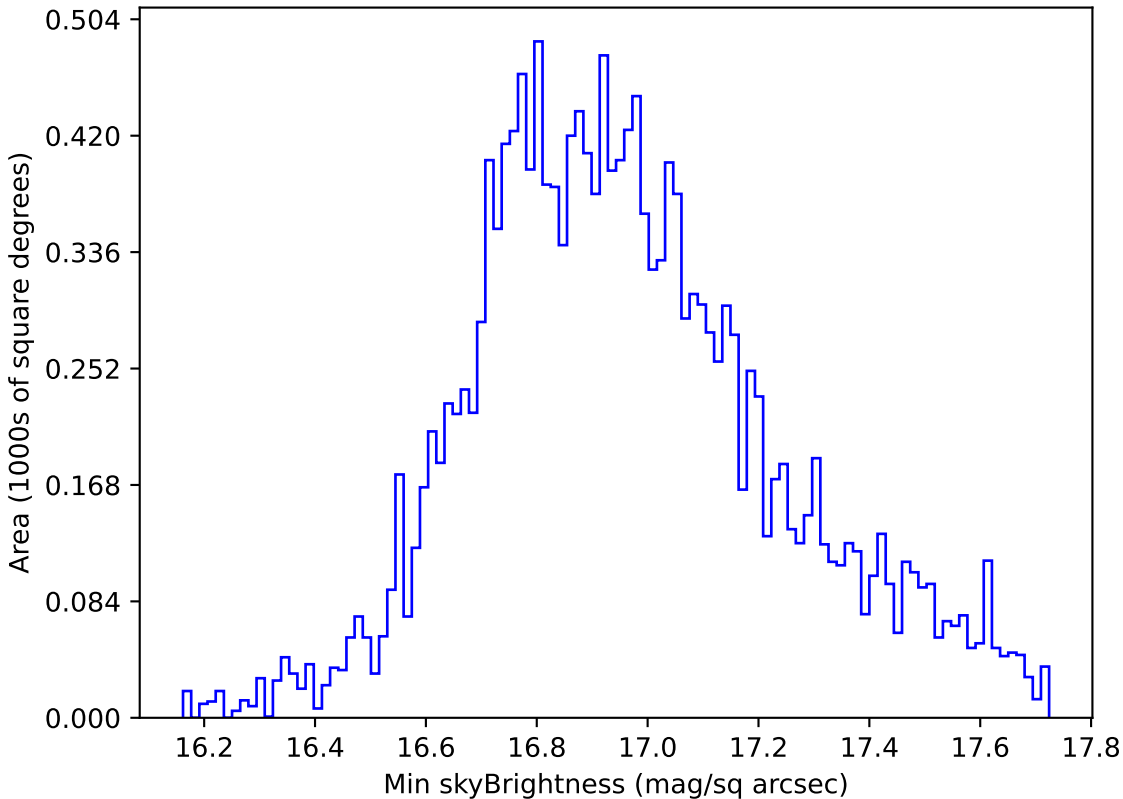
no_magell_roll_v3.4_10yrs WFD all bands: Min skyBrightness
