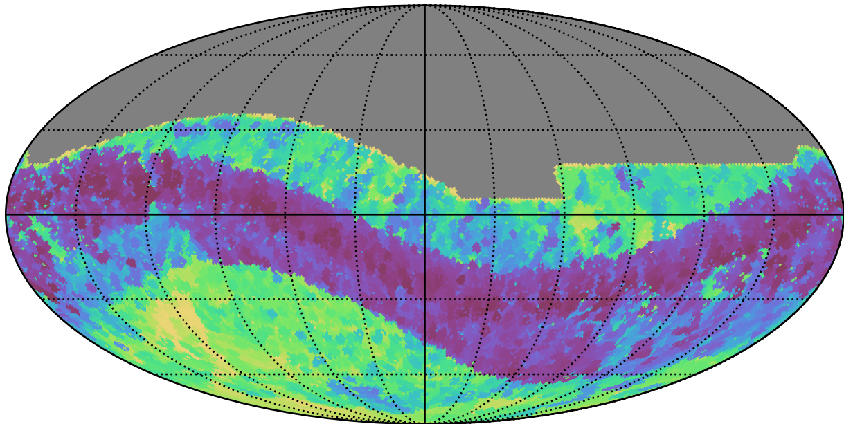
no_magell_roll_v3.4_10yrs All sky z band: Min skyBrightness
