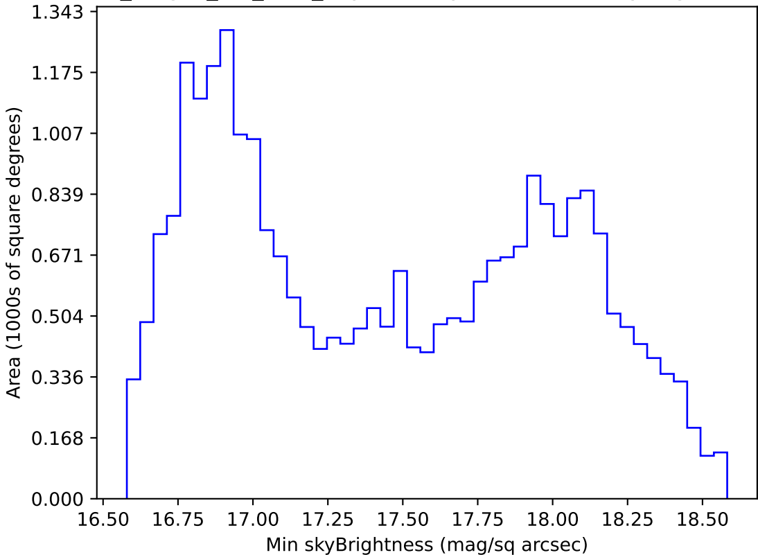
no_magell_roll_v3.4_10yrs All sky z band: Min skyBrightness
