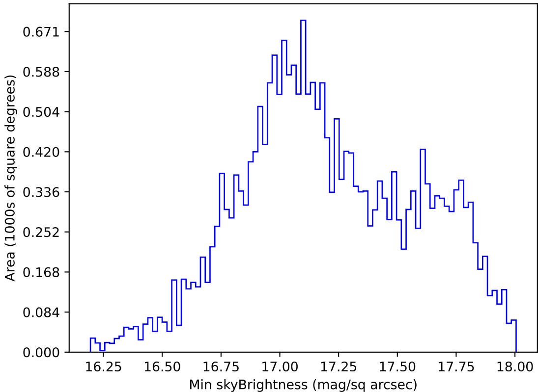
no_magell_roll_v3.4_10yrs All sky y band: Min skyBrightness
