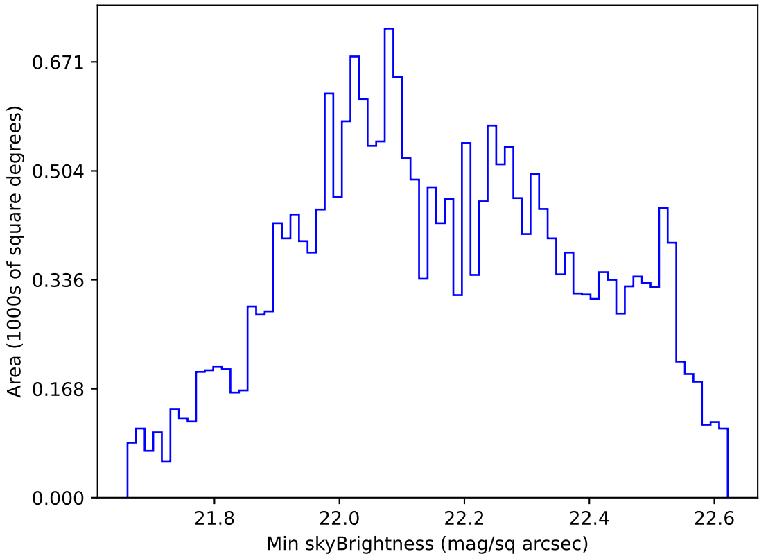
no_magell_roll_v3.4_10yrs All sky u band: Min skyBrightness
