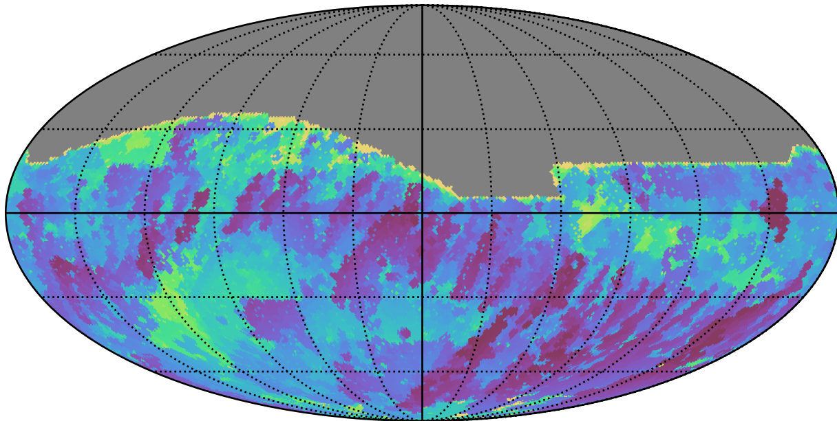
no_magell_roll_v3.4_10yrs All sky r band: Min skyBrightness
