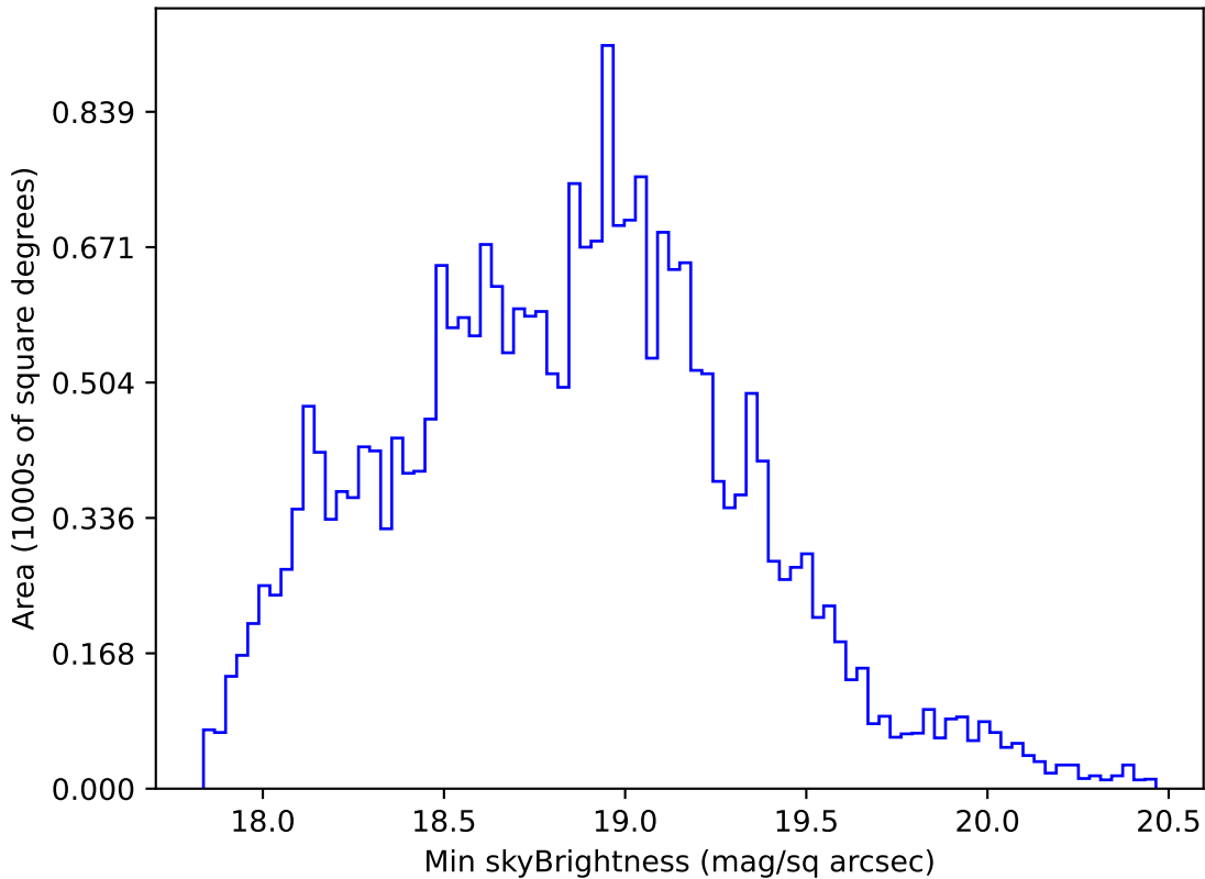
no_magell_roll_v3.4_10yrs All sky r band: Min skyBrightness
