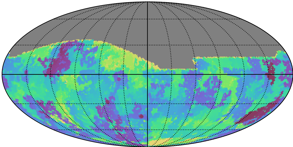
no_magell_roll_v3.4_10yrs All sky g band: Min skyBrightness
