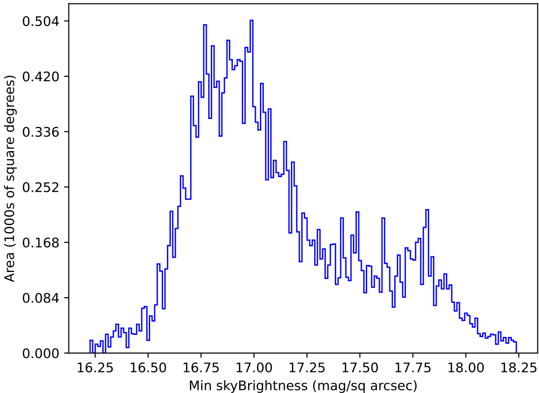
no_magell_roll_v3.4_10yrs All sky all bands: Min skyBrightness
