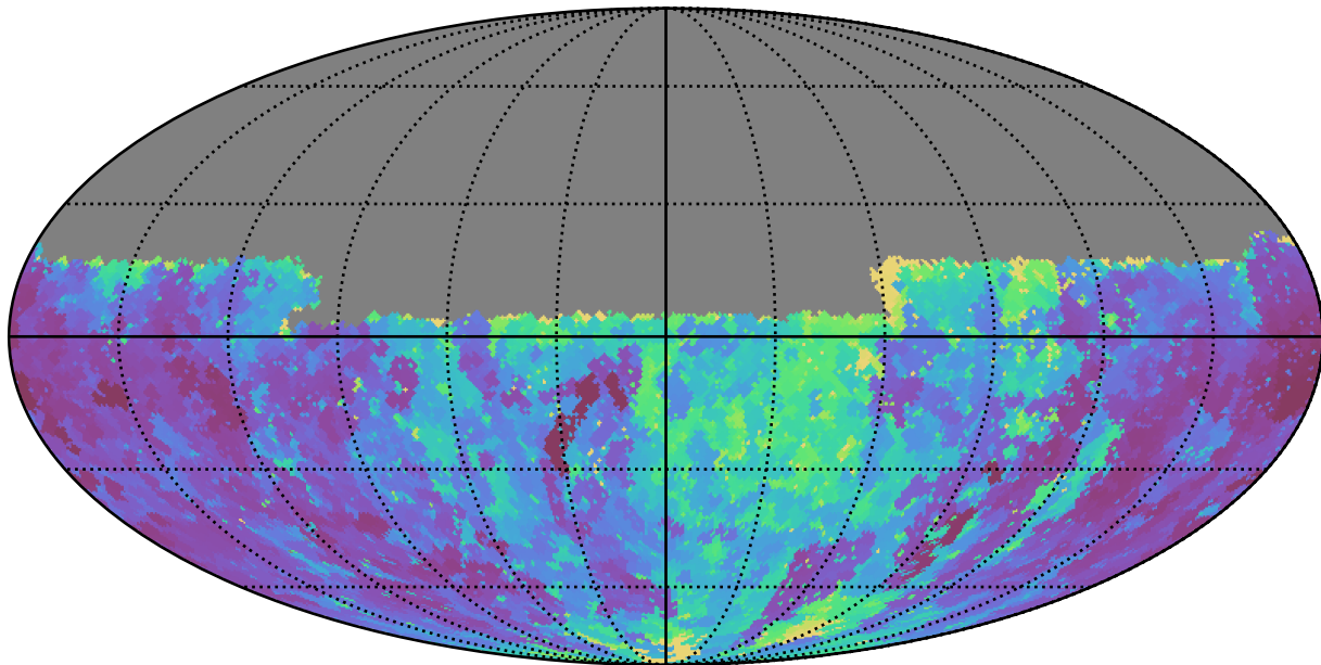
no_magell_roll_v3.4_10yrs Yr 1 u band: Min seeingEff
