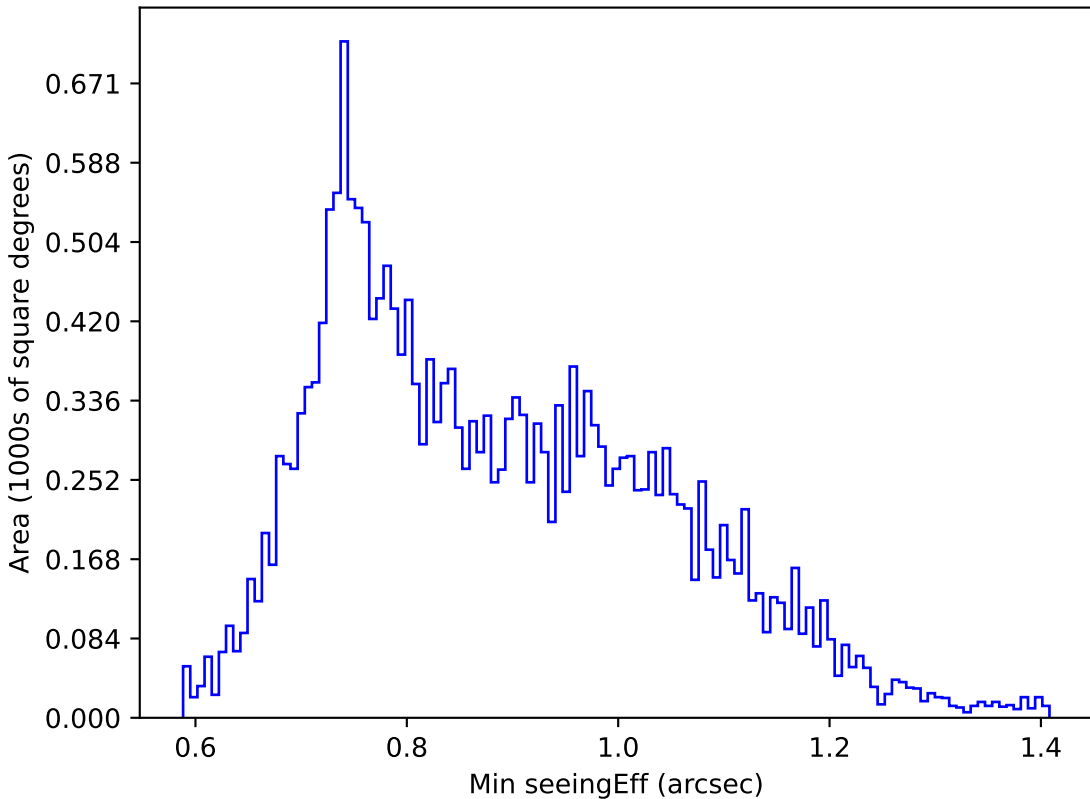
no_magell_roll_v3.4_10yrs Yr 1 u band: Min seeingEff
