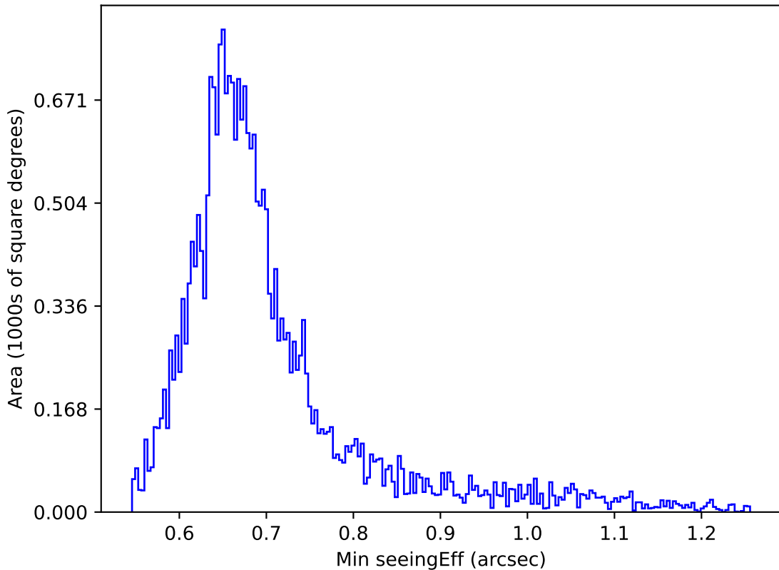
no_magell_roll_v3.4_10yrs Yr 1 i band: Min seeingEff
