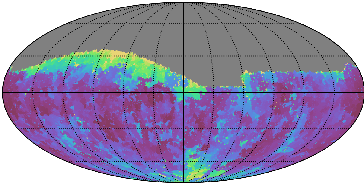
no_magell_roll_v3.4_10yrs Yr 1 g band: Min seeingEff
