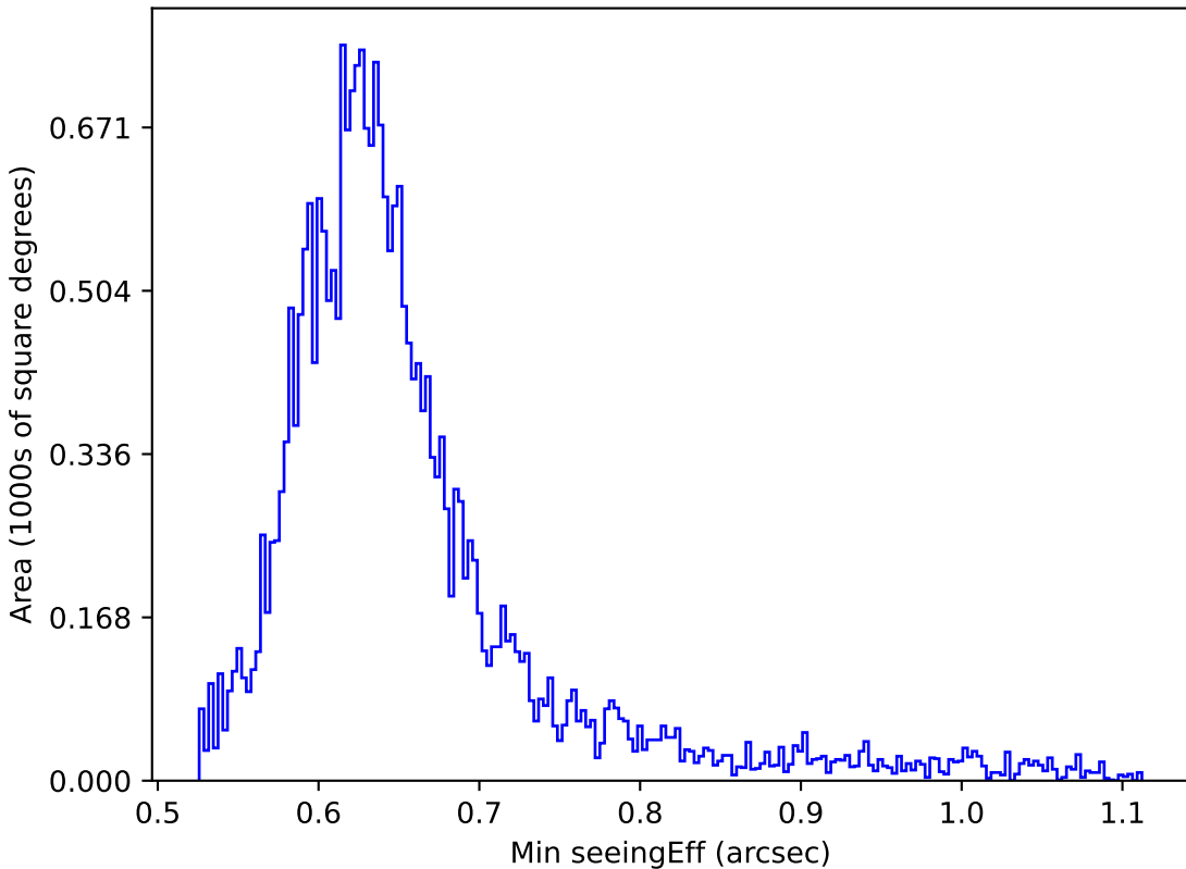
no_magell_roll_v3.4_10yrs Yr 1 all bands: Min seeingEff
