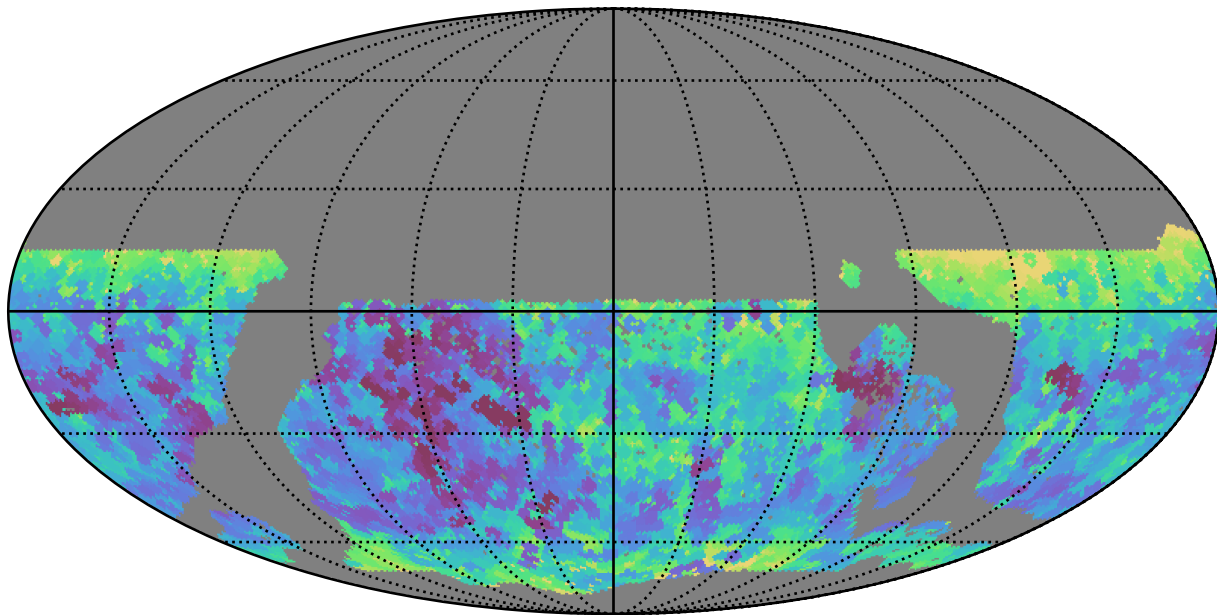
no_magell_roll_v3.4_10yrs WFD z band: Min seeingEff
